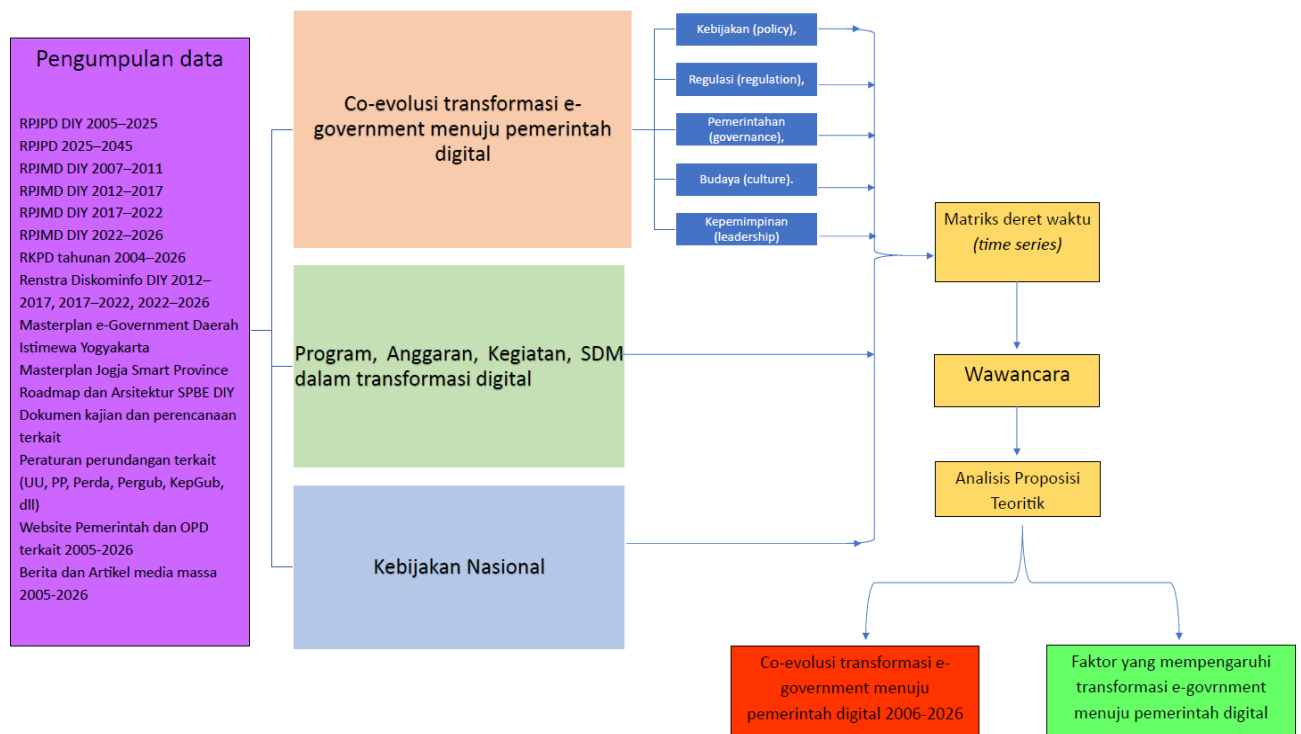
Figure 2 Analysis flow
