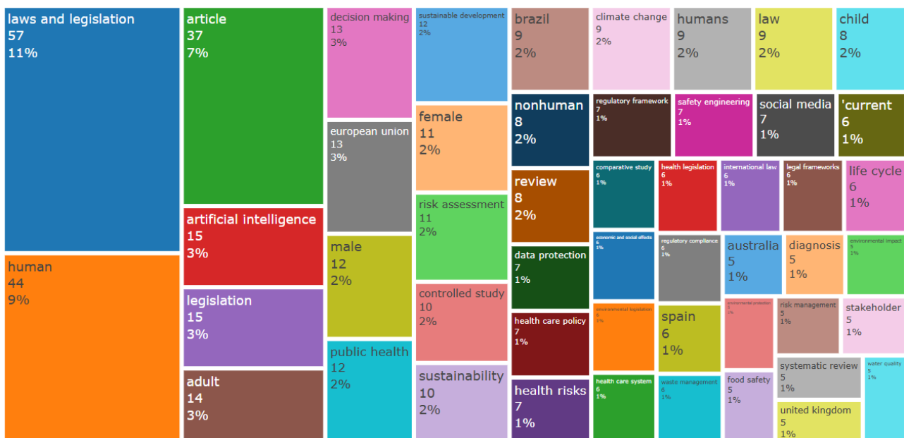
Figure 8 TreeMap
