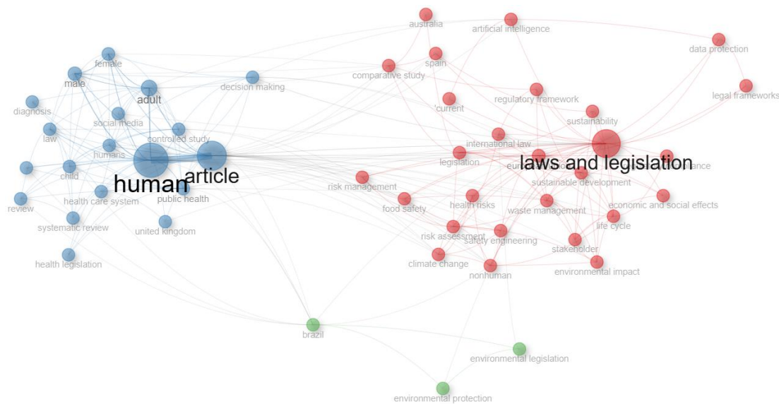
Figure 9 Co-occurrence network
